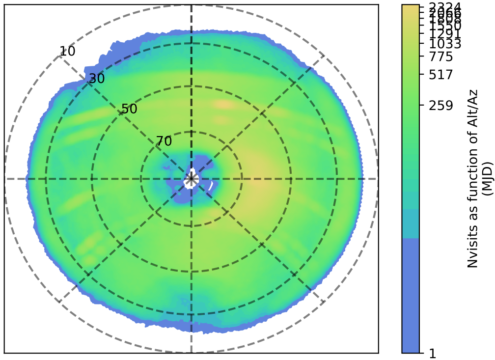
too_elab_heavy_r64_d2_griz_v3.4_10yrs z: Nvisits as function of Alt/Az
