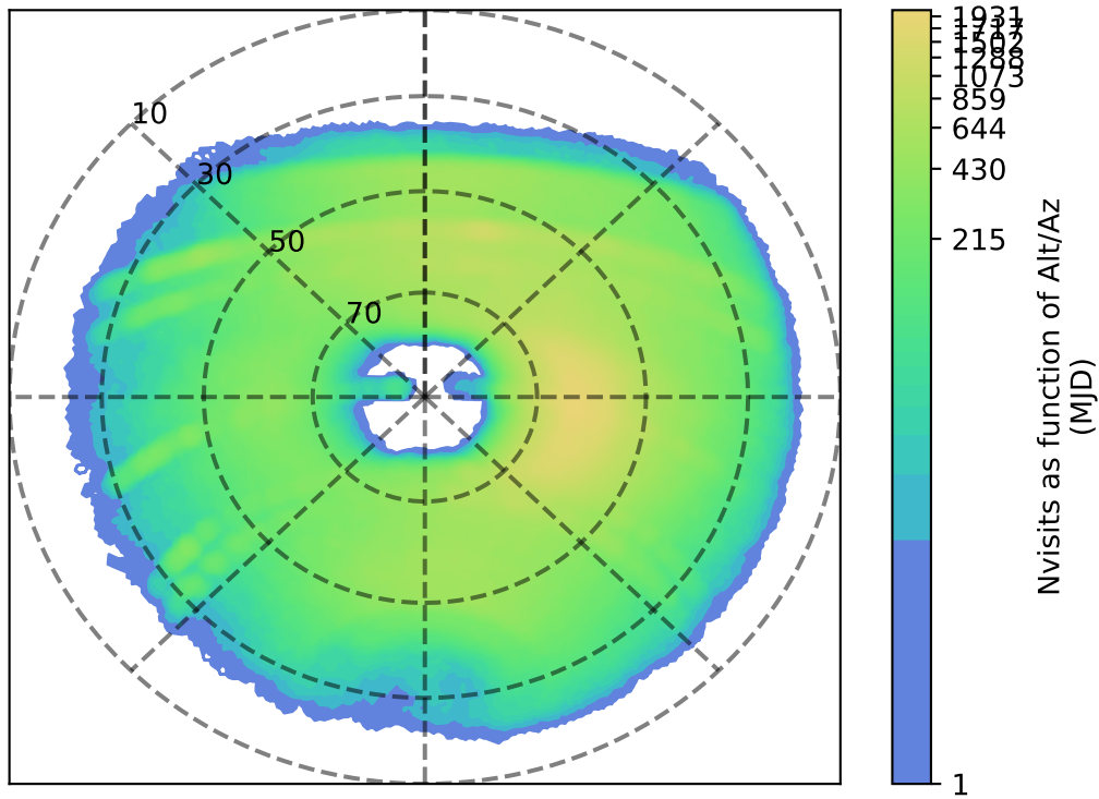
too_elab_heavy_r64_d2_griz_v3.4_10yrs y: Nvisits as function of Alt/Az
