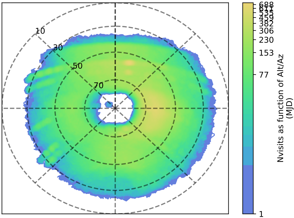
too_elab_heavy_r64_d2_griz_v3.4_10yrs u: Nvisits as function of Alt/Az
