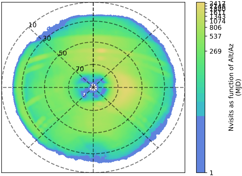
too_elab_heavy_r64_d2_griz_v3.4_10yrs r: Nvisits as function of Alt/Az
