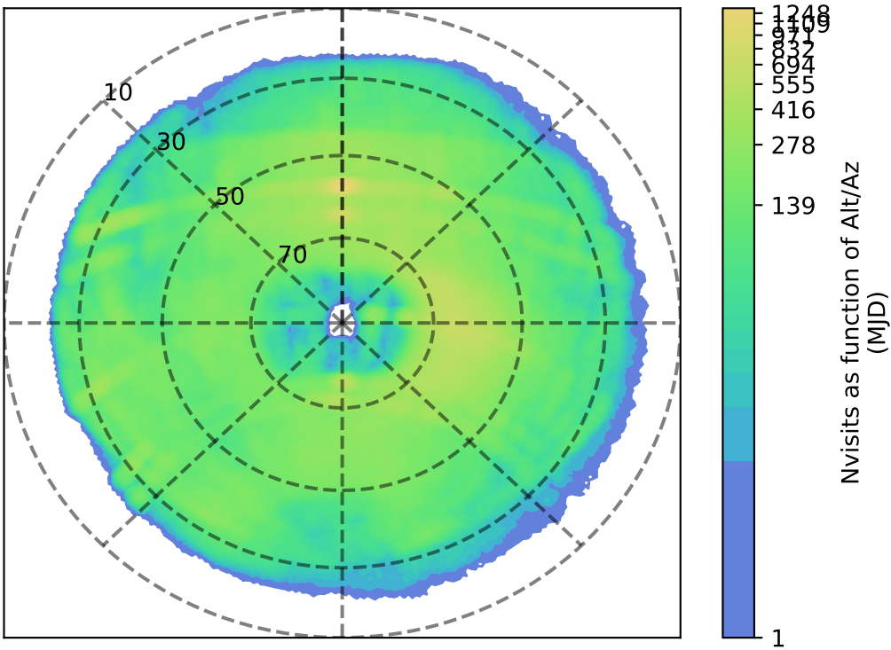
too_elab_heavy_r64_d2_griz_v3.4_10yrs g: Nvisits as function of Alt/Az
