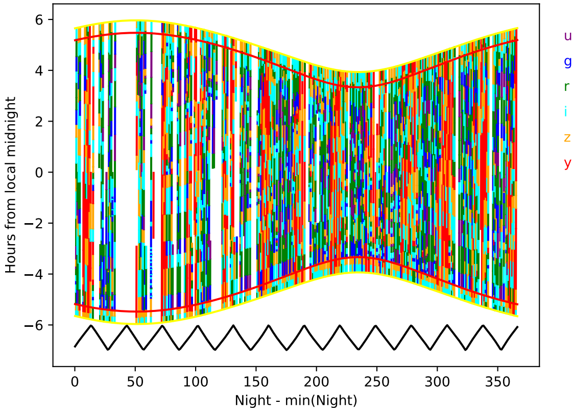
too_elab_heavy_r64_d2_griz_v3.4_10yrs year 8-9: Hourglass
