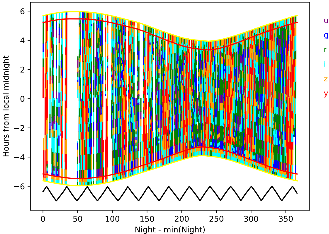
too_elab_heavy_r64_d2_griz_v3.4_10yrs year 6-7: Hourglass
