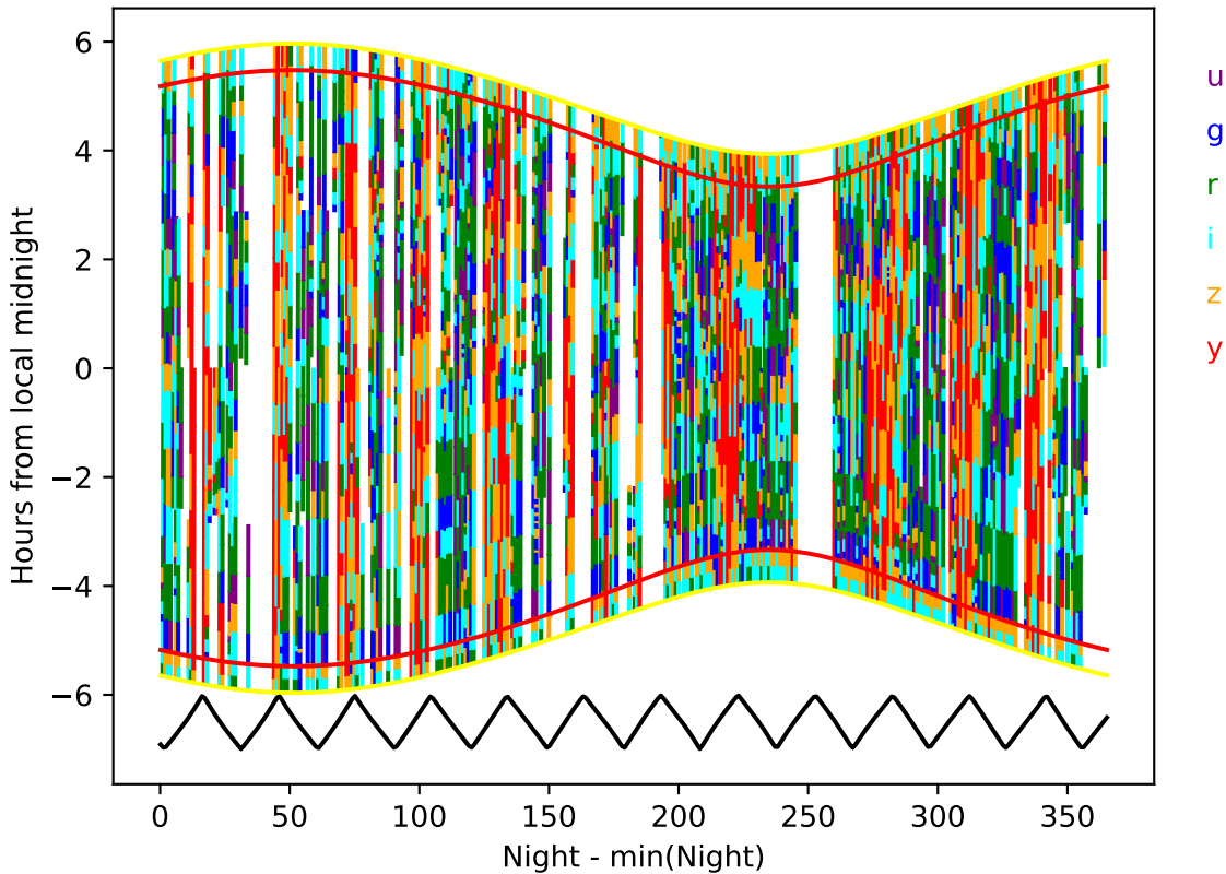
too_elab_heavy_r64_d2_griz_v3.4_10yrs year 5-6: Hourglass
