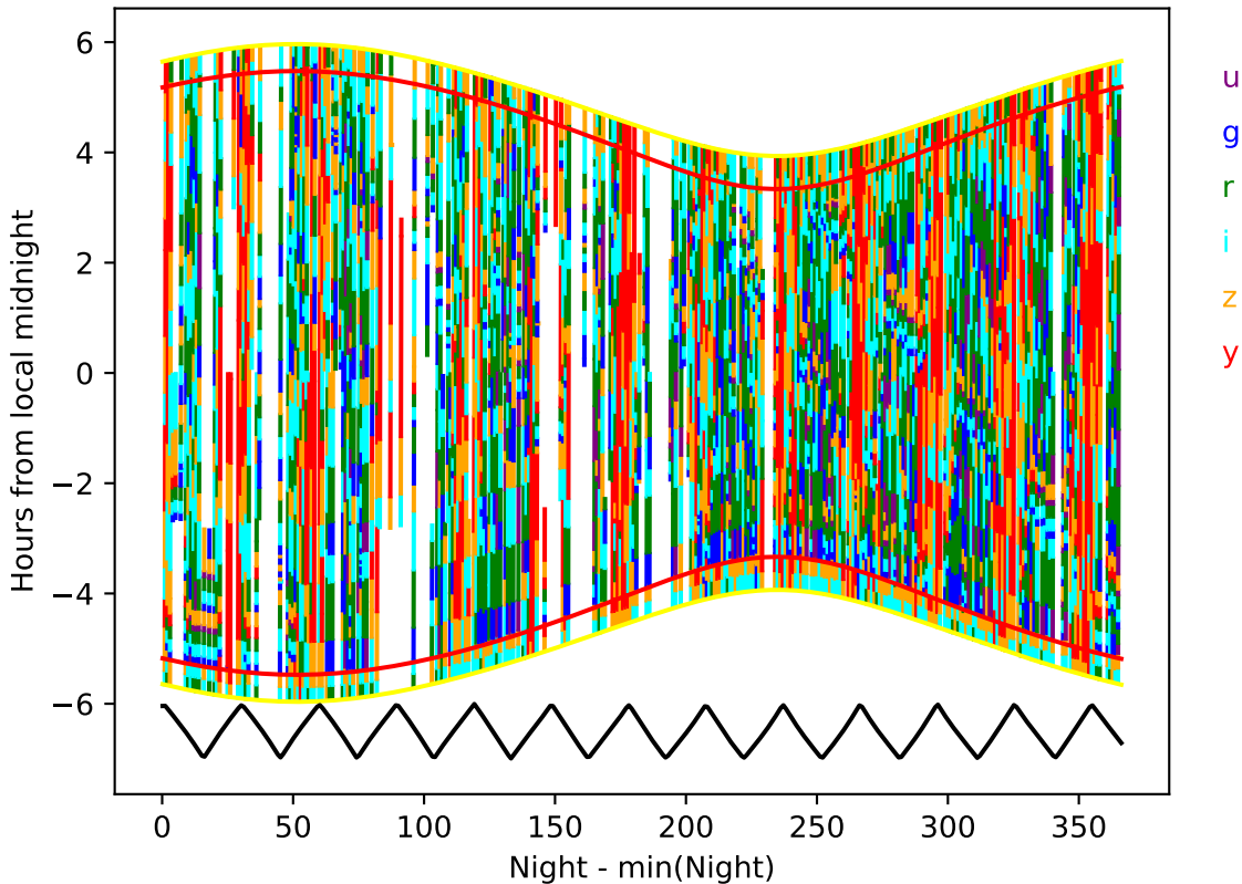
too_elab_heavy_r64_d2_griz_v3.4_10yrs year 1-2: Hourglass
