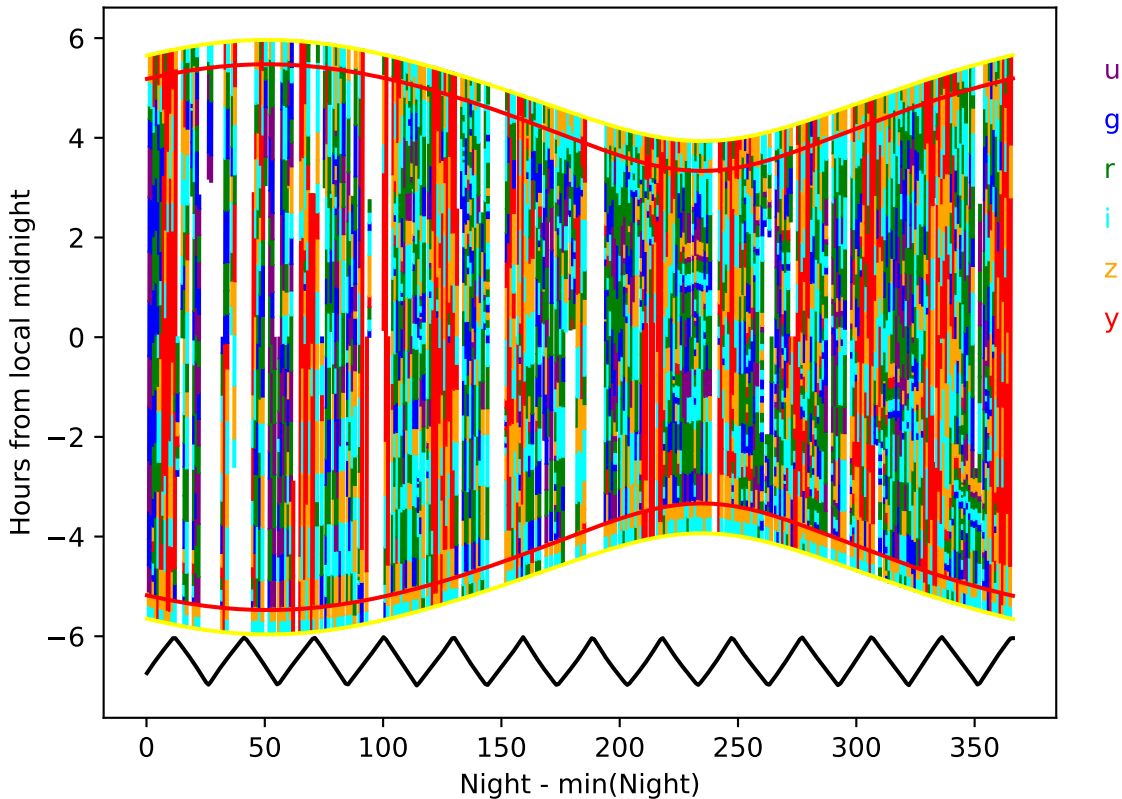
too_elab_heavy_r64_d2_griz_v3.4_10yrs year 0-1: Hourglass
