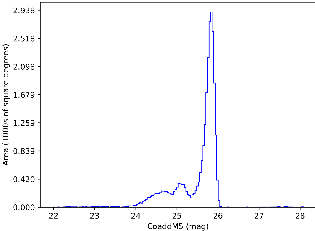
too_elab_heavy_r64_d2_griz_v3.4_10yrs z: CoaddM5
