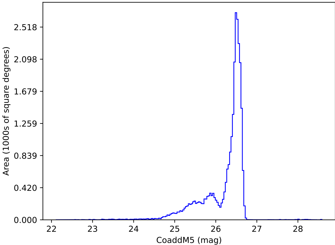
too_elab_heavy_r64_d2_griz_v3.4_10yrs i: CoaddM5
