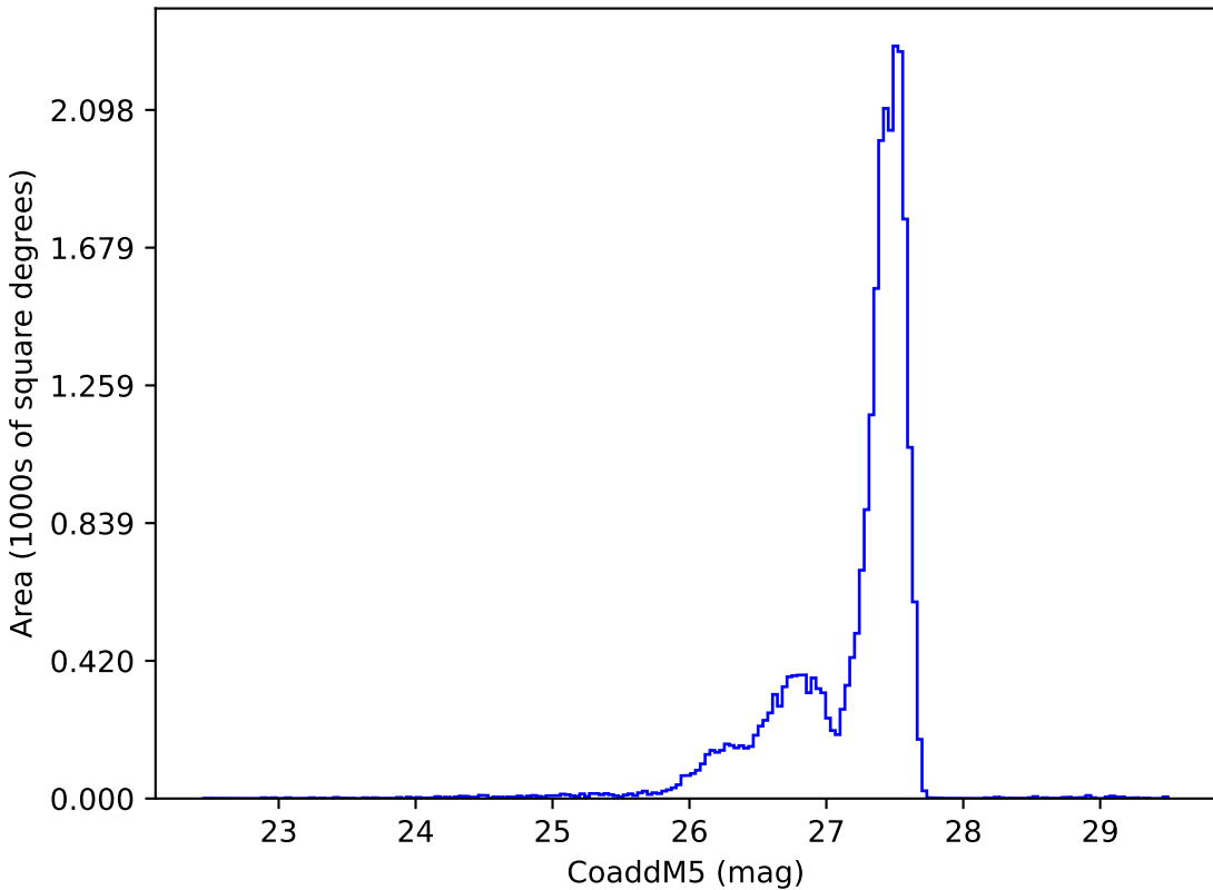
too_elab_heavy_r64_d2_griz_v3.4_10yrs : CoaddM5
