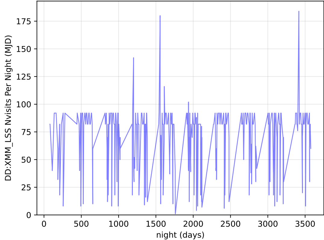
too_elab_heavy_r64_d2_griz_v3.4_10yrs all bands: DD:XMM_LSS Nvisits Per Night
