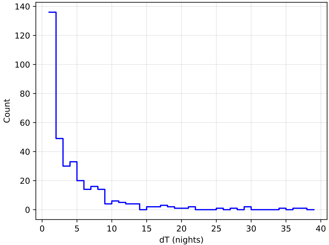
too_elab_heavy_r64_d2_griz_v3.4_10yrs all bands: DD:WFD Delta Nights Histogram
