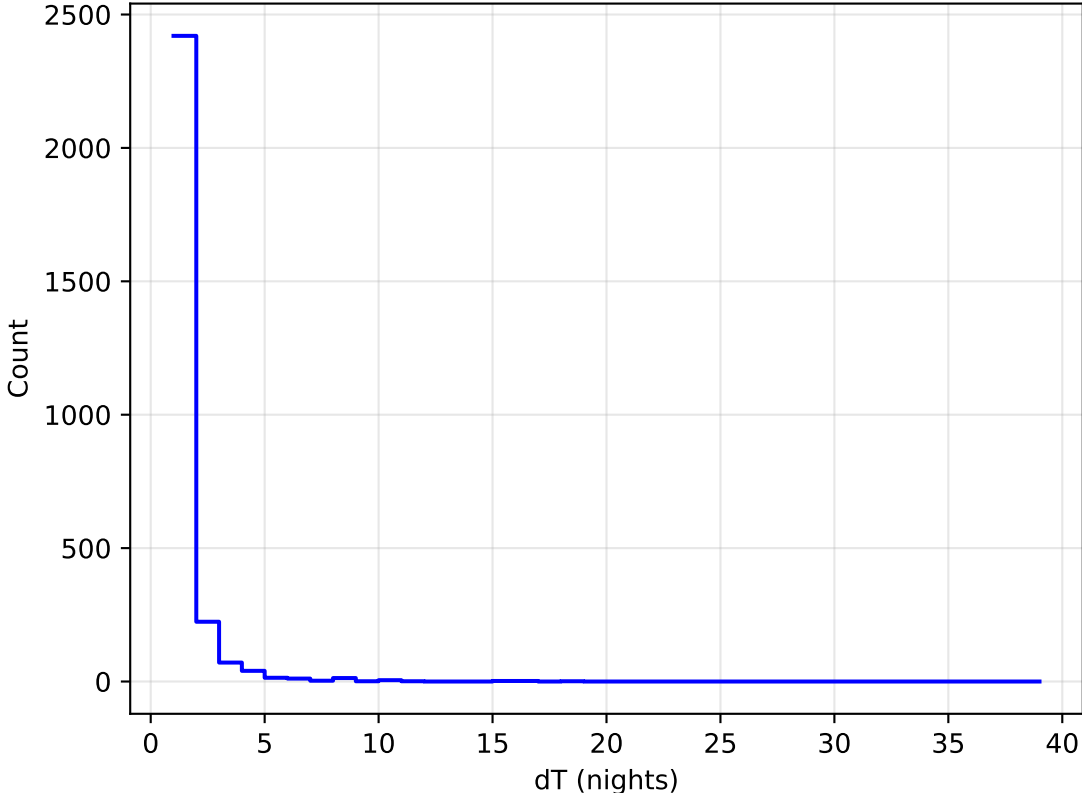
too_elab_heavy_r64_d2_griz_v3.4_10yrs all bands: DD:WFD Delta Nights Histogram
