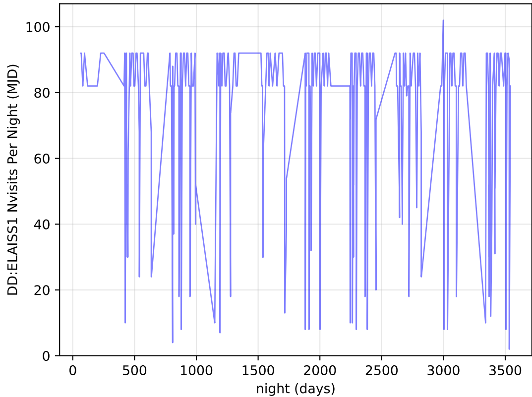
too_elab_heavy_r64_d2_griz_v3.4_10yrs all bands: DD:ELAISS1 Nvisits Per Night
