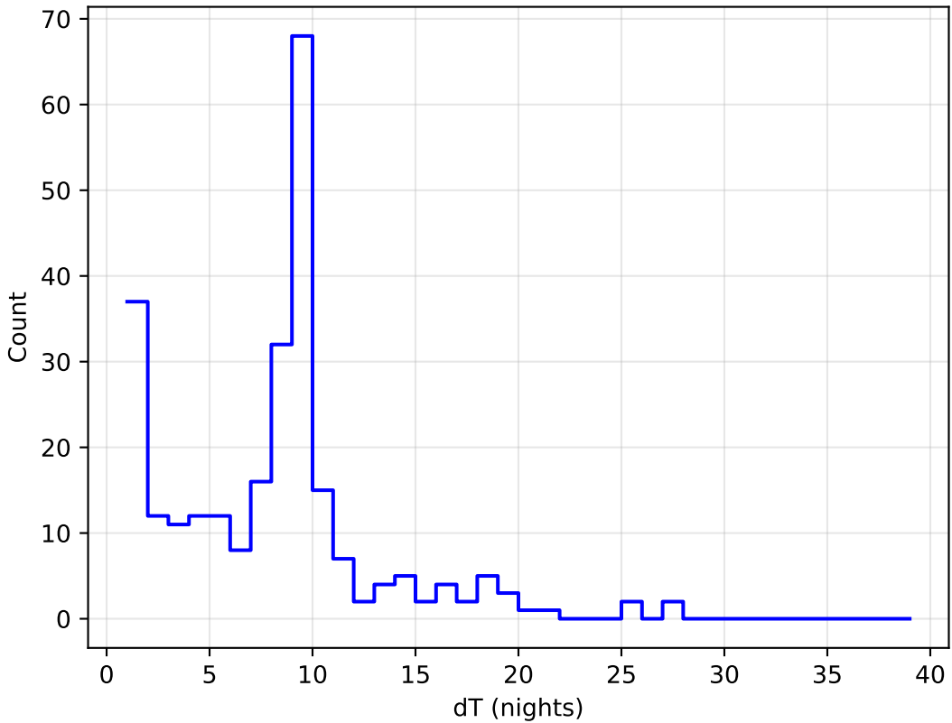
too_elab_heavy_r64_d2_griz_v3.4_10yrs all bands: DD:ELAISS1 Delta Nights Histogram
