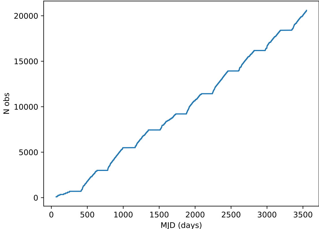
too_elab_heavy_r64_d2_griz_v3.4_10yrs all bands: DD:ELAISS1 Cumulative NVisits
