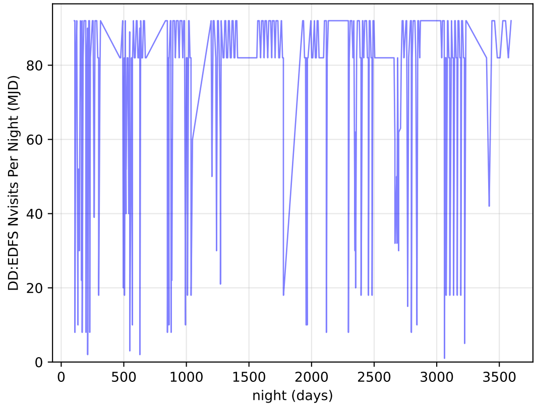
too_elab_heavy_r64_d2_griz_v3.4_10yrs all bands: DD:EDFS Nvisits Per Night
