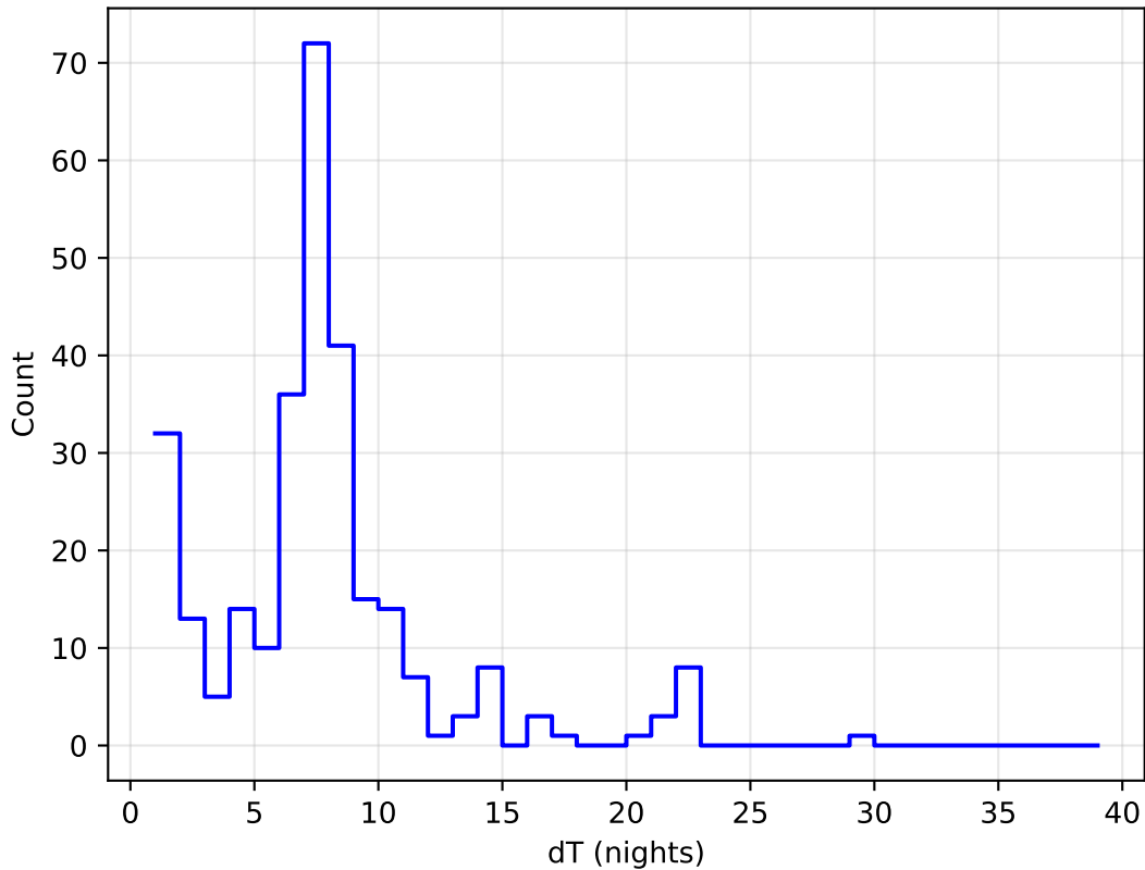
too_elab_heavy_r64_d2_griz_v3.4_10yrs all bands: DD:EDFS Delta Nights Histogram
