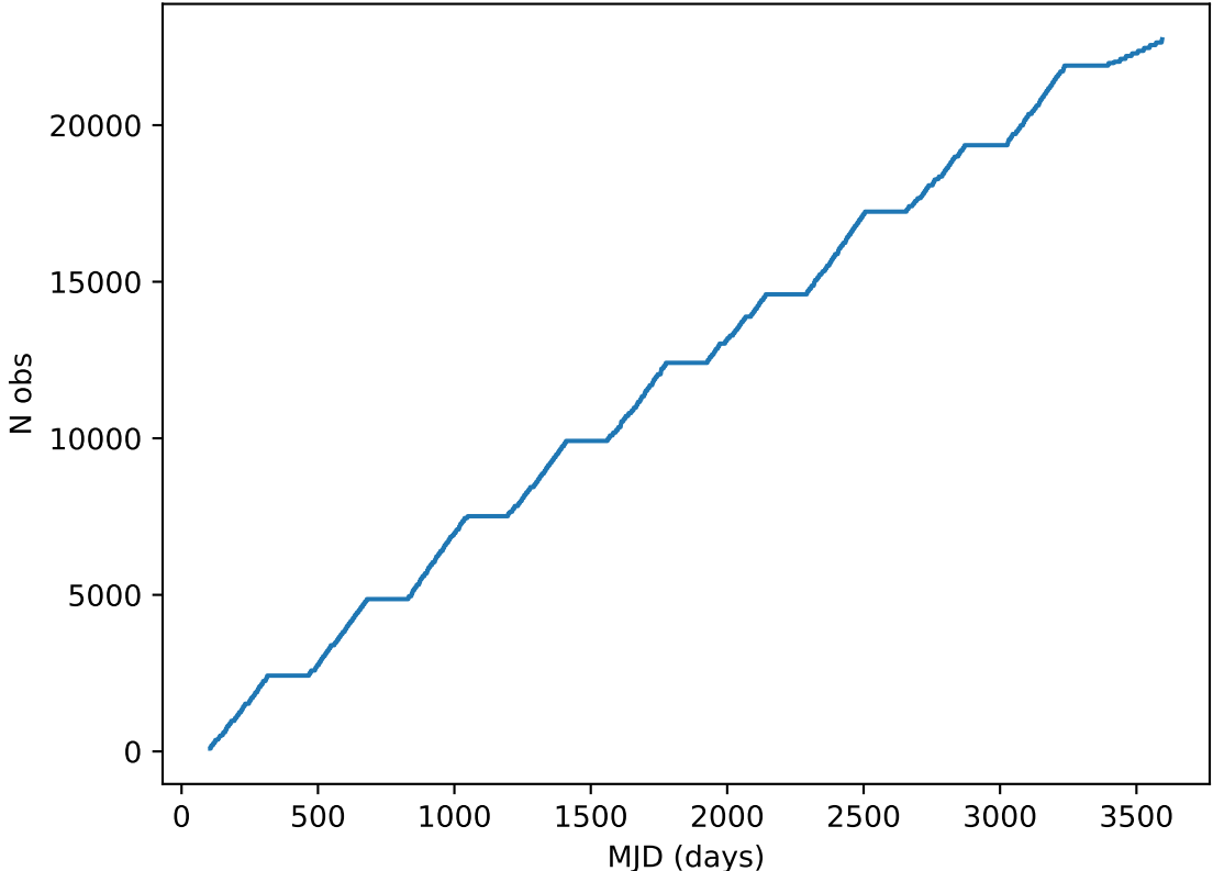
too_elab_heavy_r64_d2_griz_v3.4_10yrs all bands: DD:EDFS Cumulative NVisits
