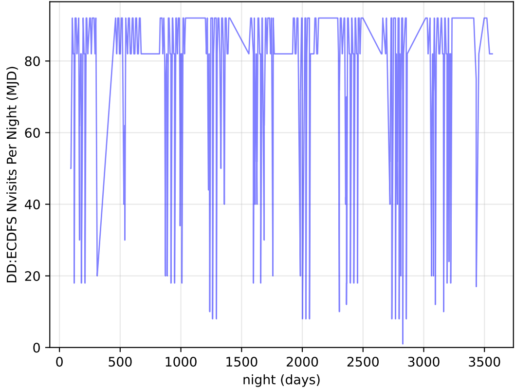
too_elab_heavy_r64_d2_griz_v3.4_10yrs all bands: DD:ECDFS Nvisits Per Night
