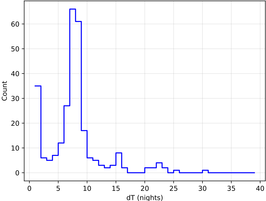
too_elab_heavy_r64_d2_griz_v3.4_10yrs all bands: DD:ECDFS Delta Nights Histogram
