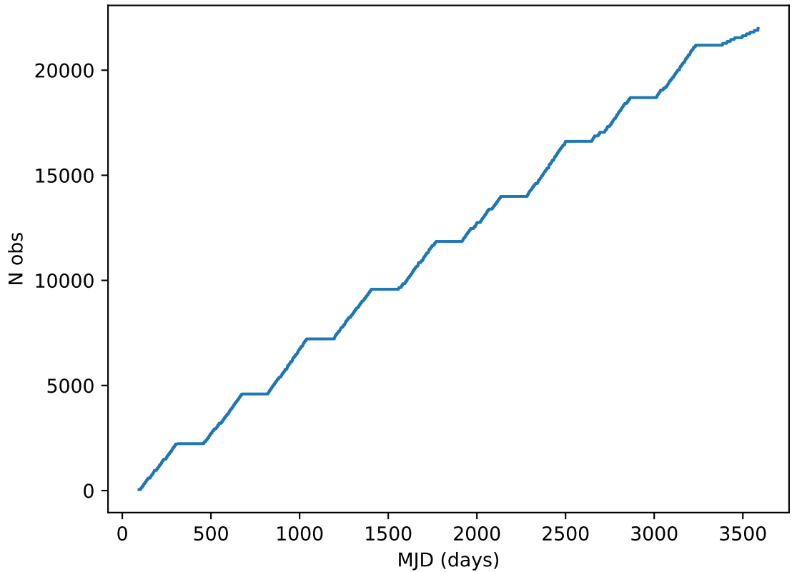
too_elab_heavy_r64_d2_griz_v3.4_10yrs all bands: DD:ECDFS Cumulative NVisits
