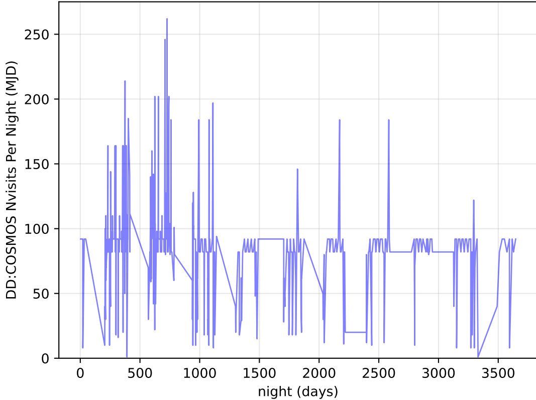
too_elab_heavy_r64_d2_griz_v3.4_10yrs all bands: DD:COSMOS Nvisits Per Night
