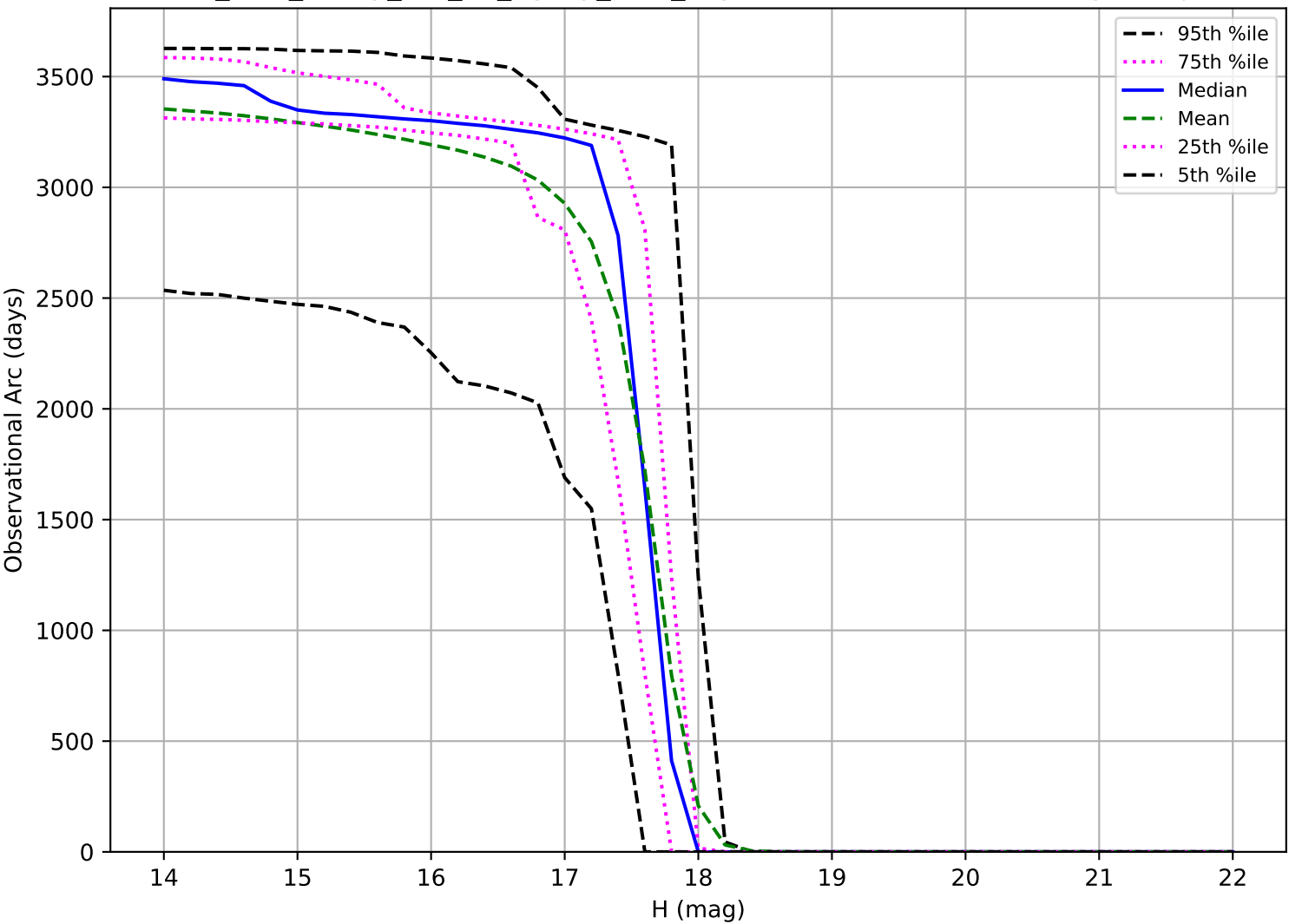
too_elab_heavy_r32_d3_ugrizy_v3.4_10yrs: Observational Arc Length Trojan
