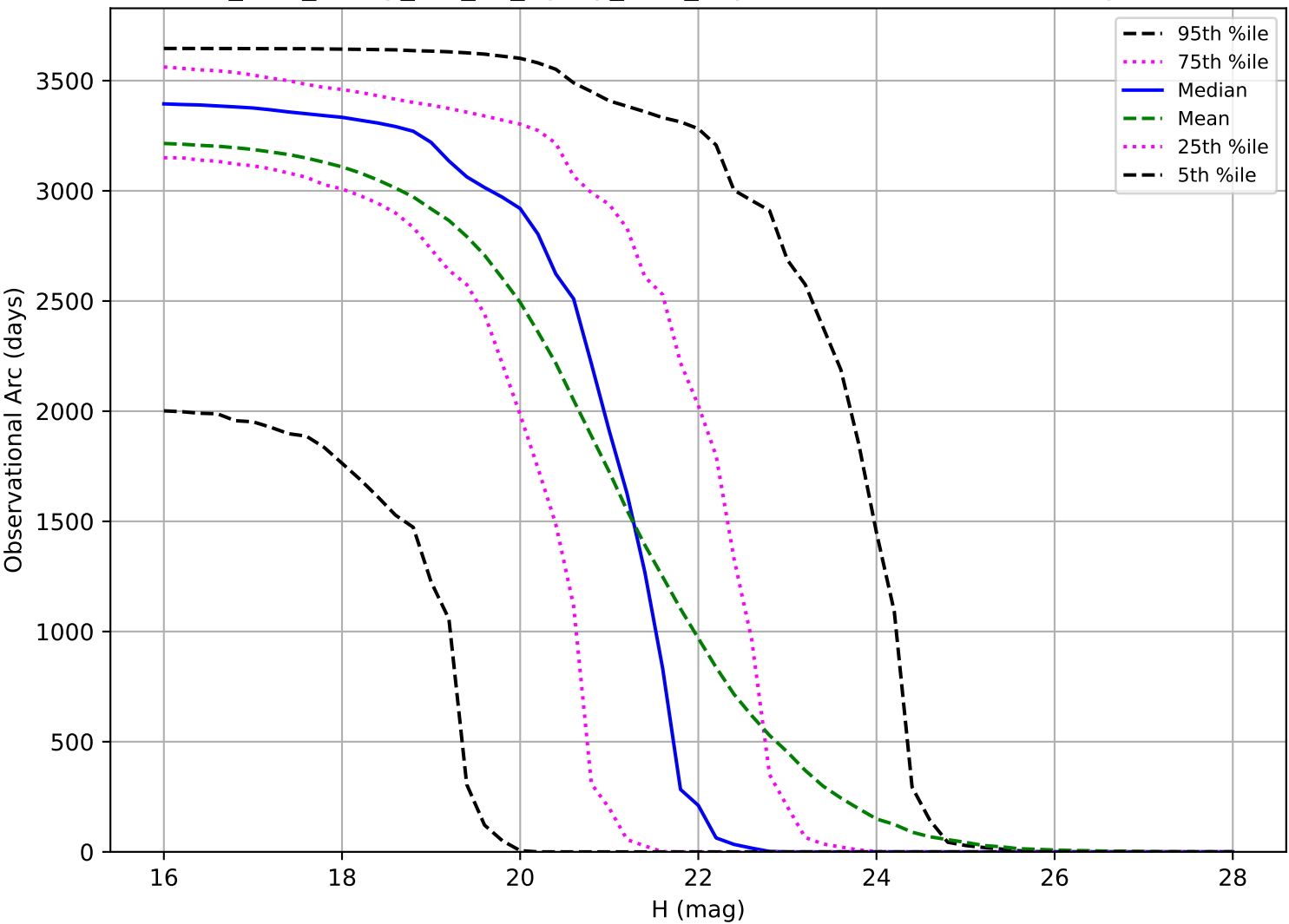
too_elab_heavy_r32_d3_ugrizy_v3.4_10yrs: Observational Arc Length PHA
