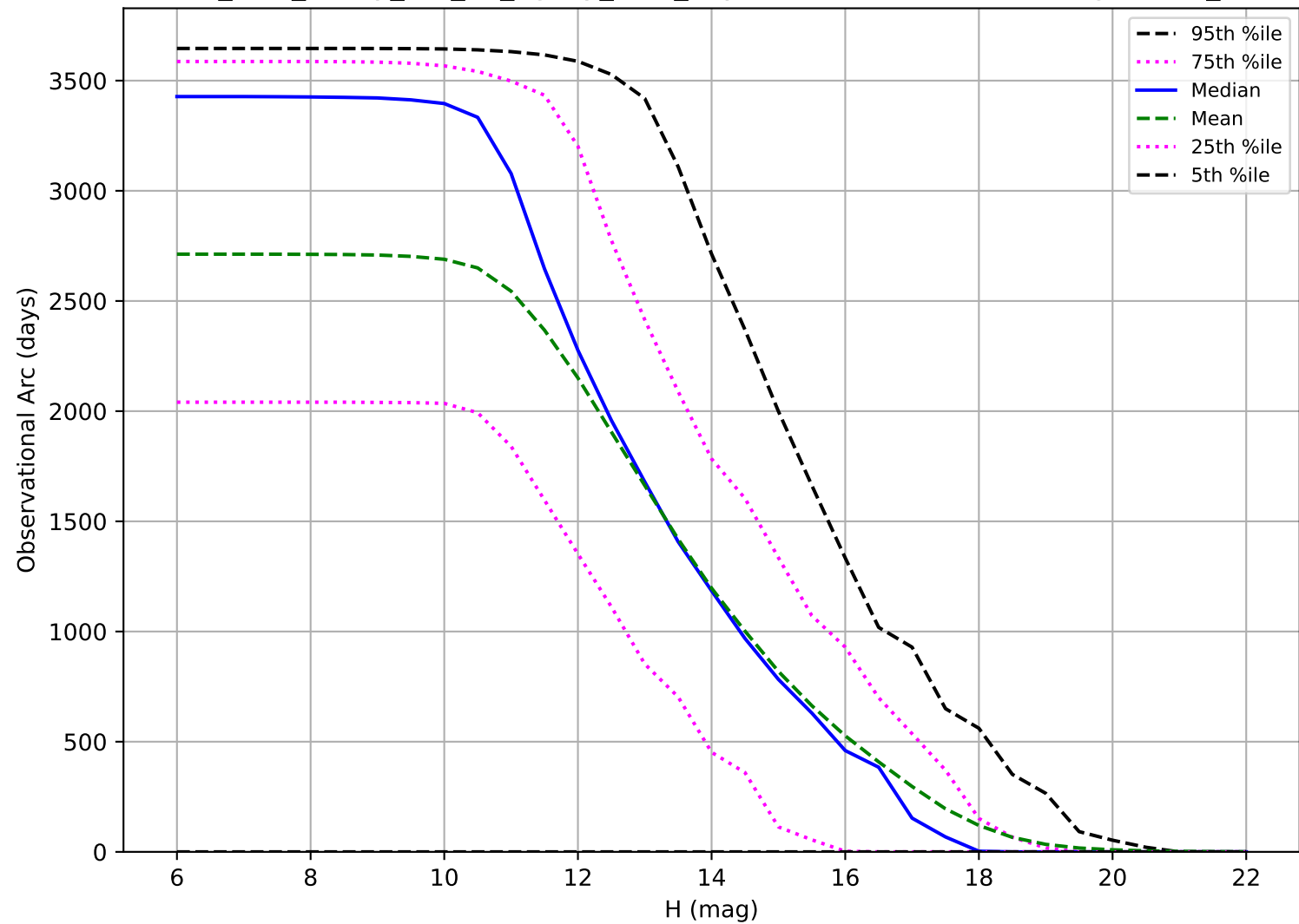
too_elab_heavy_r32_d3_ugrizy_v3.4_10yrs: Observational Arc Length OCC_r5
