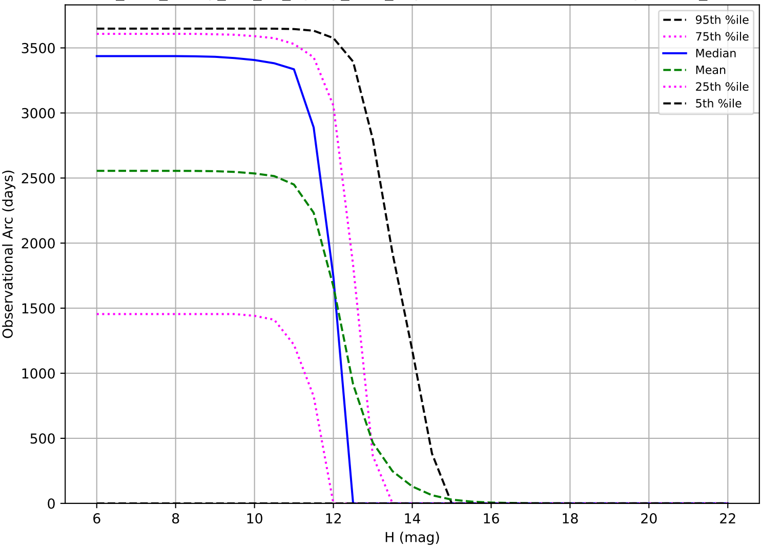
too_elab_heavy_r32_d3_ugrizy_v3.4_10yrs: Observational Arc Length OCC_r20
