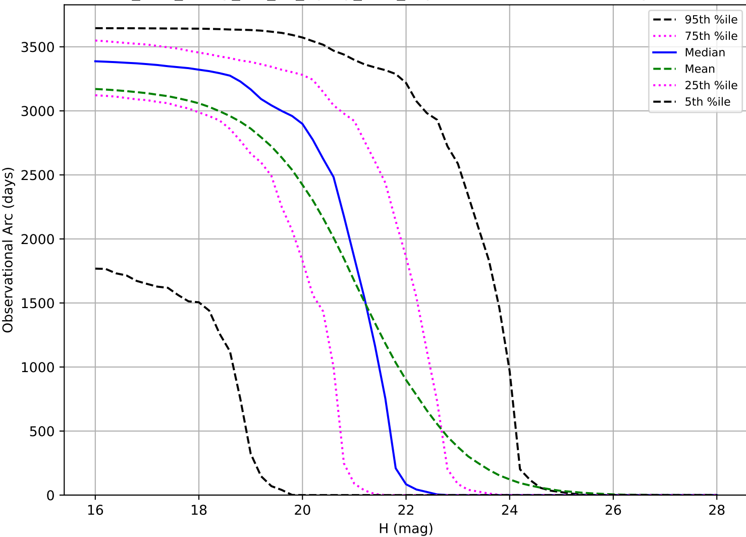
too_elab_heavy_r32_d3_ugrizy_v3.4_10yrs: Observational Arc Length NEO
