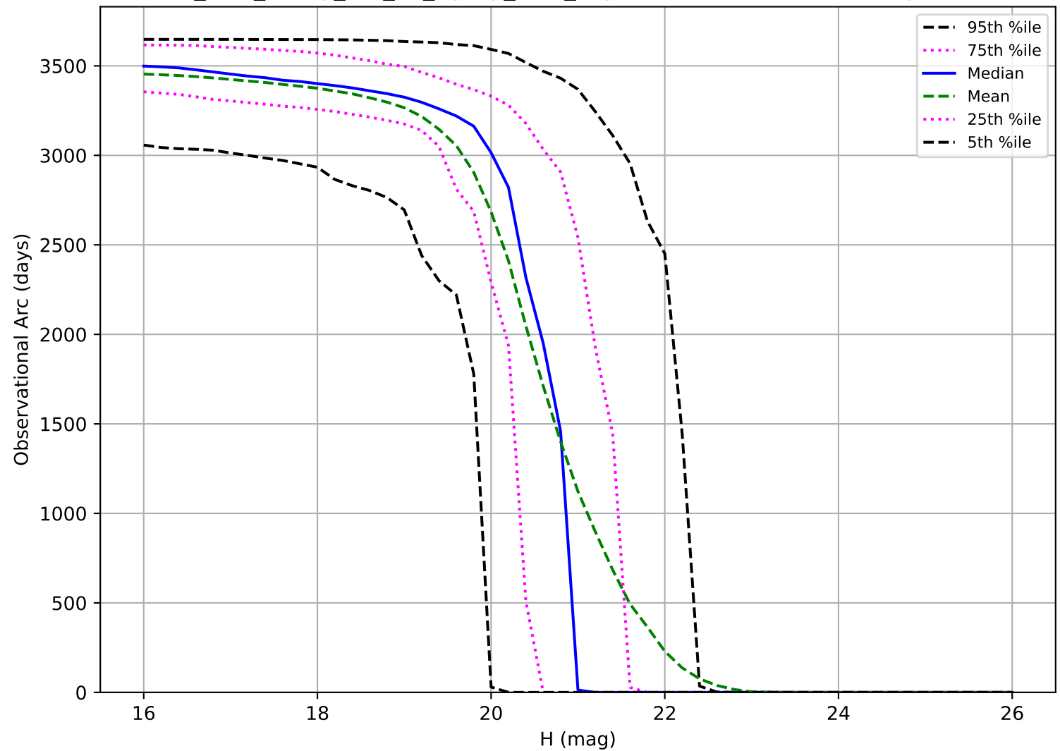
too_elab_heavy_r32_d3_ugrizy_v3.4_10yrs: Observational Arc Length MBA
