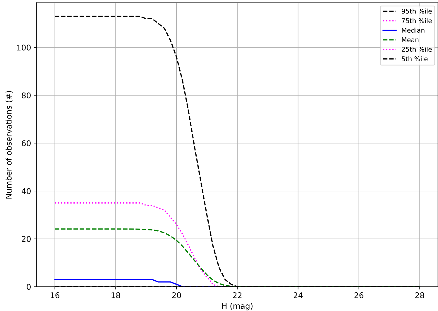
too_elab_heavy_r32_d3_ugrizy_v3.4_10yrs: Number of observations Vatira
