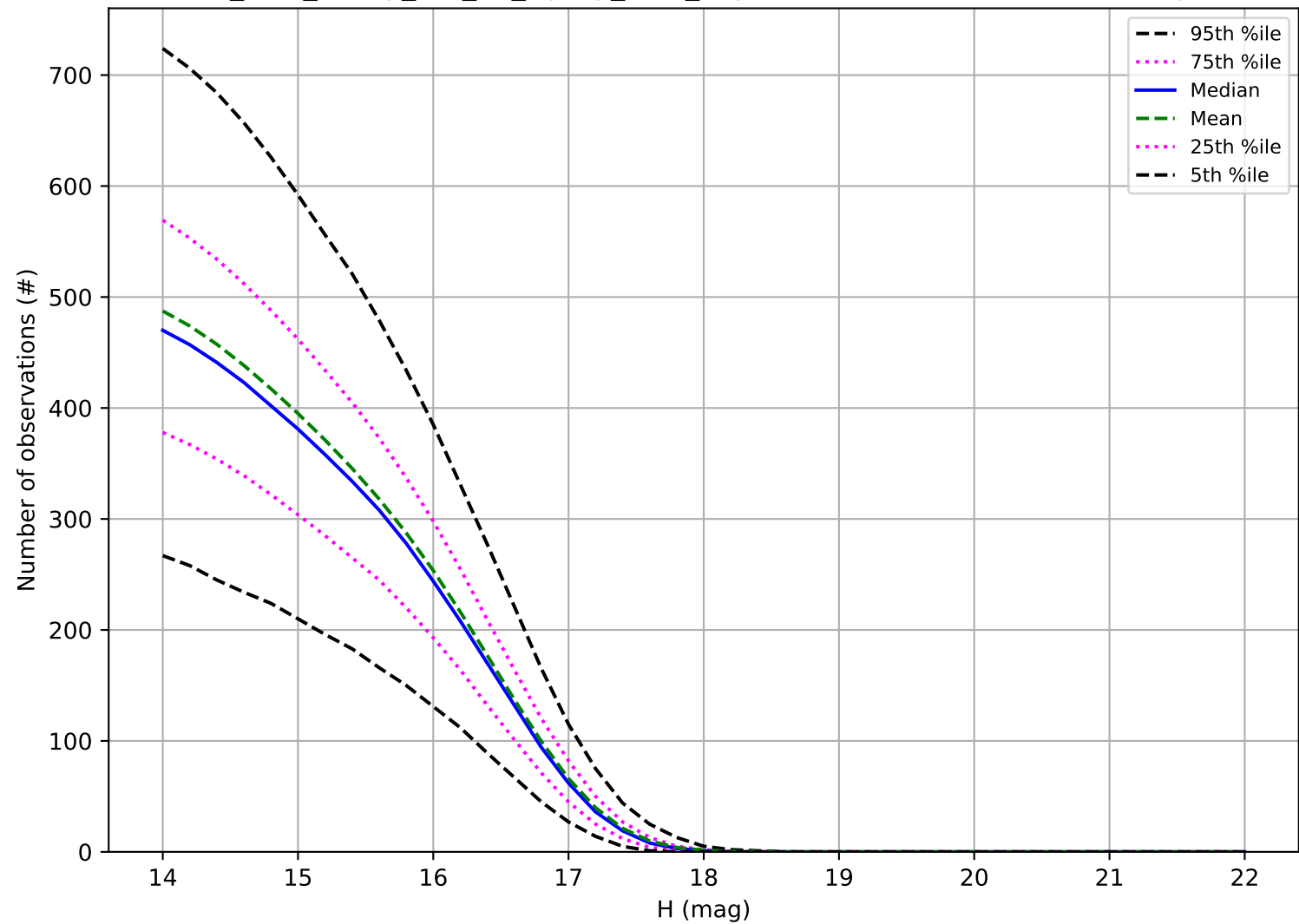
too_elab_heavy_r32_d3_ugrizy_v3.4_10yrs: Number of observations Trojan
