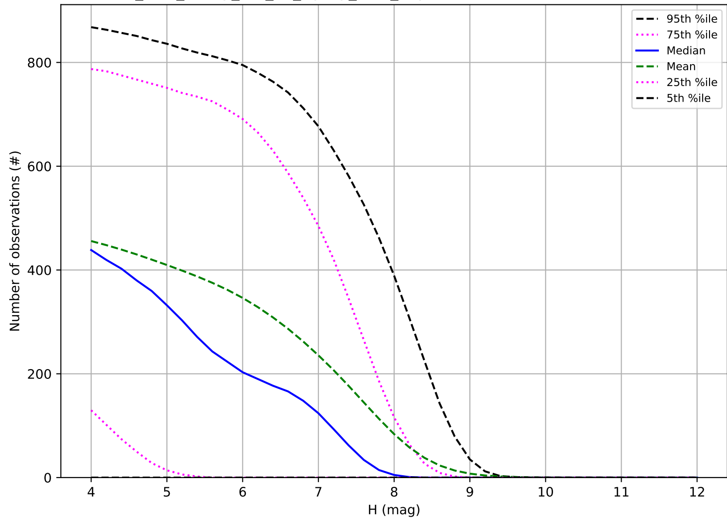
too_elab_heavy_r32_d3_ugrizy_v3.4_10yrs: Number of observations TNO
