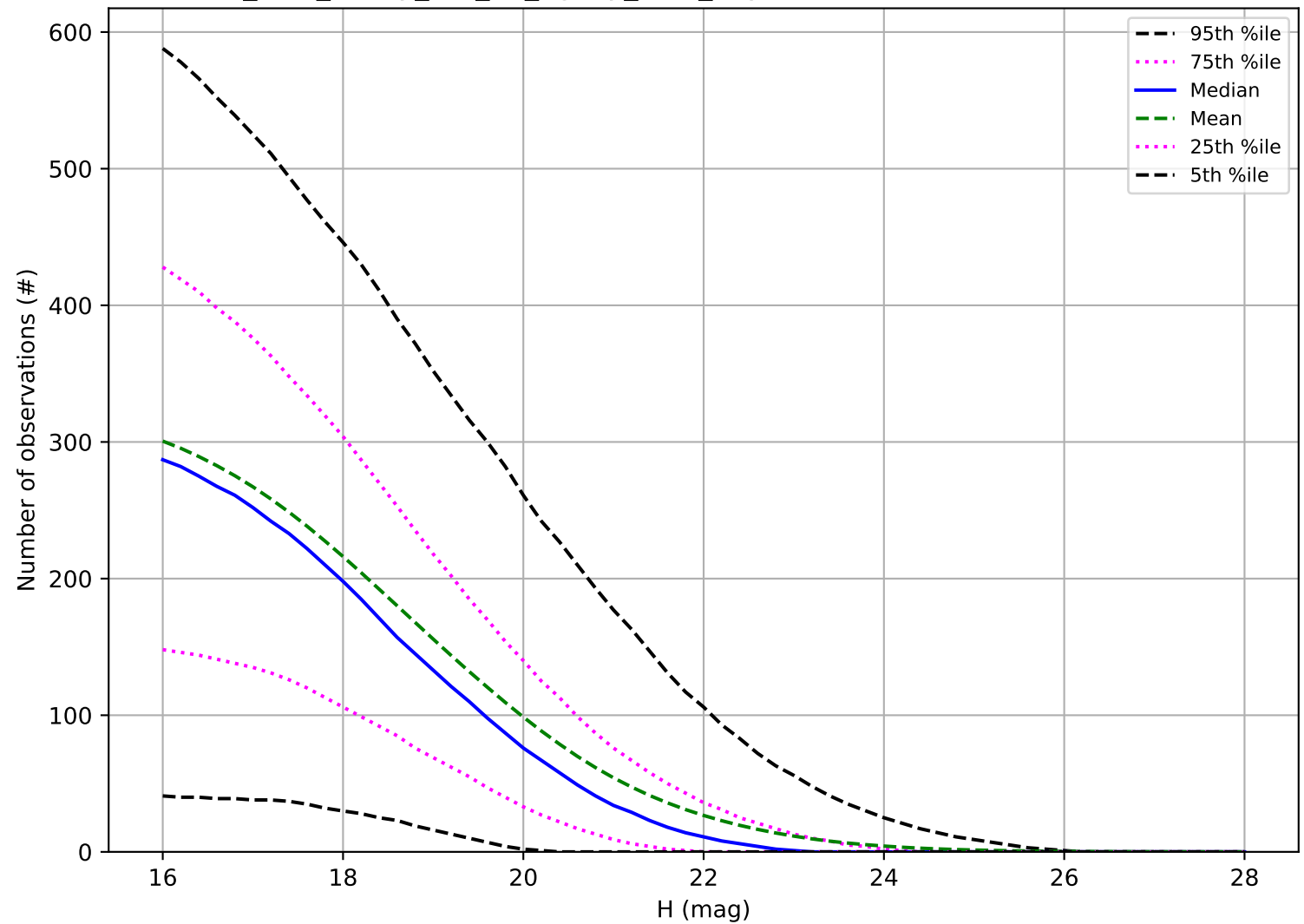
too_elab_heavy_r32_d3_ugrizy_v3.4_10yrs: Number of observations PHA
