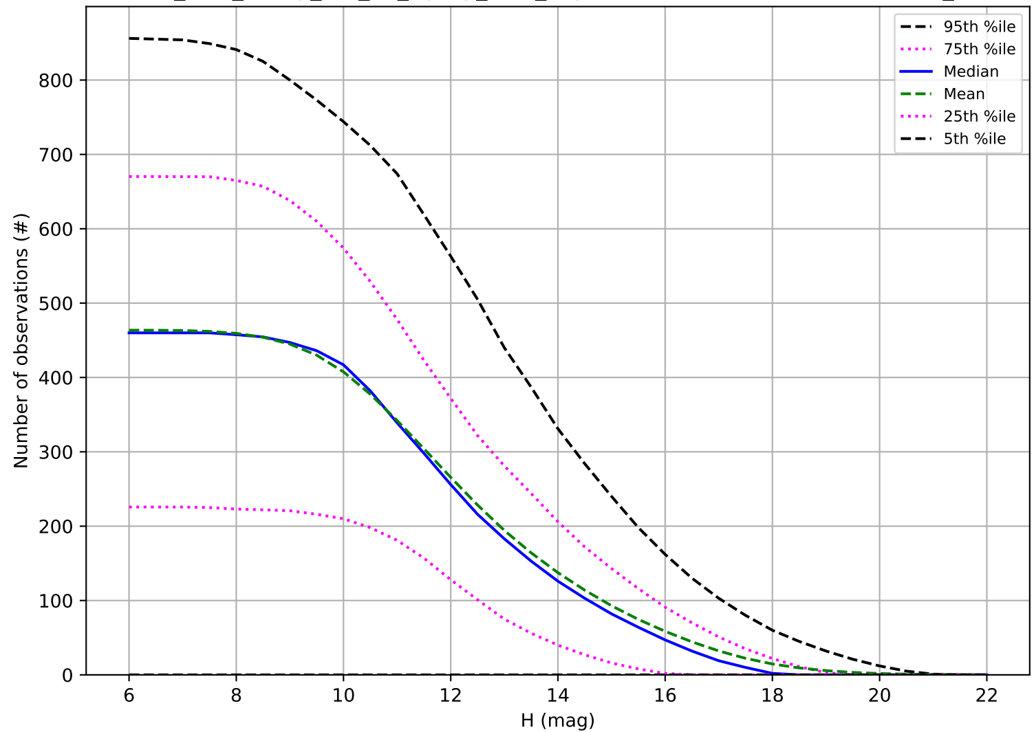
too_elab_heavy_r32_d3_ugrizy_v3.4_10yrs: Number of observations OCC_r5
