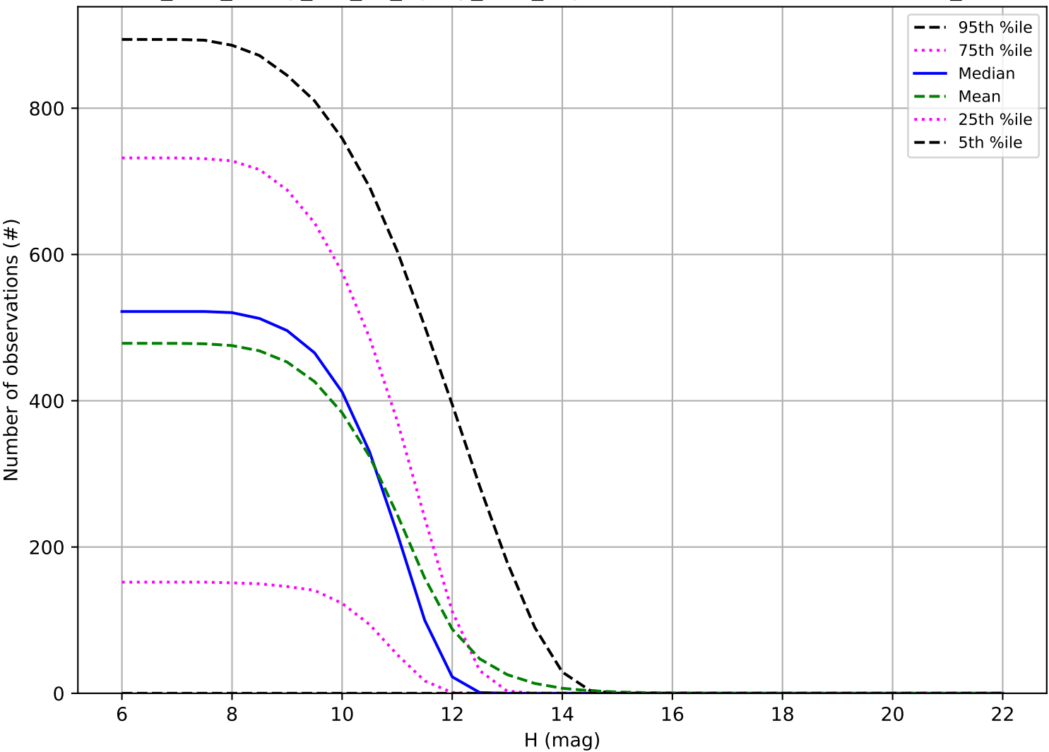
too_elab_heavy_r32_d3_ugrizy_v3.4_10yrs: Number of observations OCC_r20
