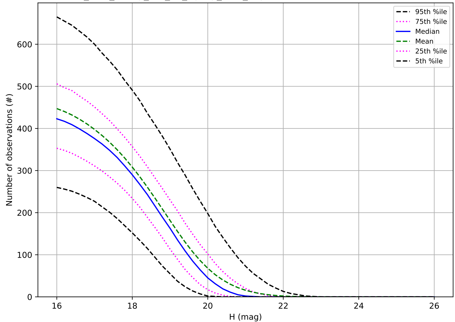
too_elab_heavy_r32_d3_ugrizy_v3.4_10yrs: Number of observations MBA
