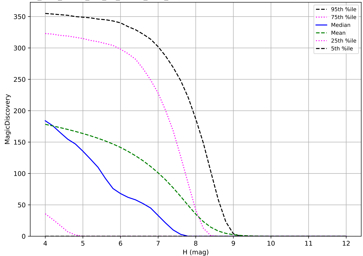
too_elab_heavy_r32_d3_ugrizy_v3.4_10yrs: TNO 6 detections in 60 nights detection loss
