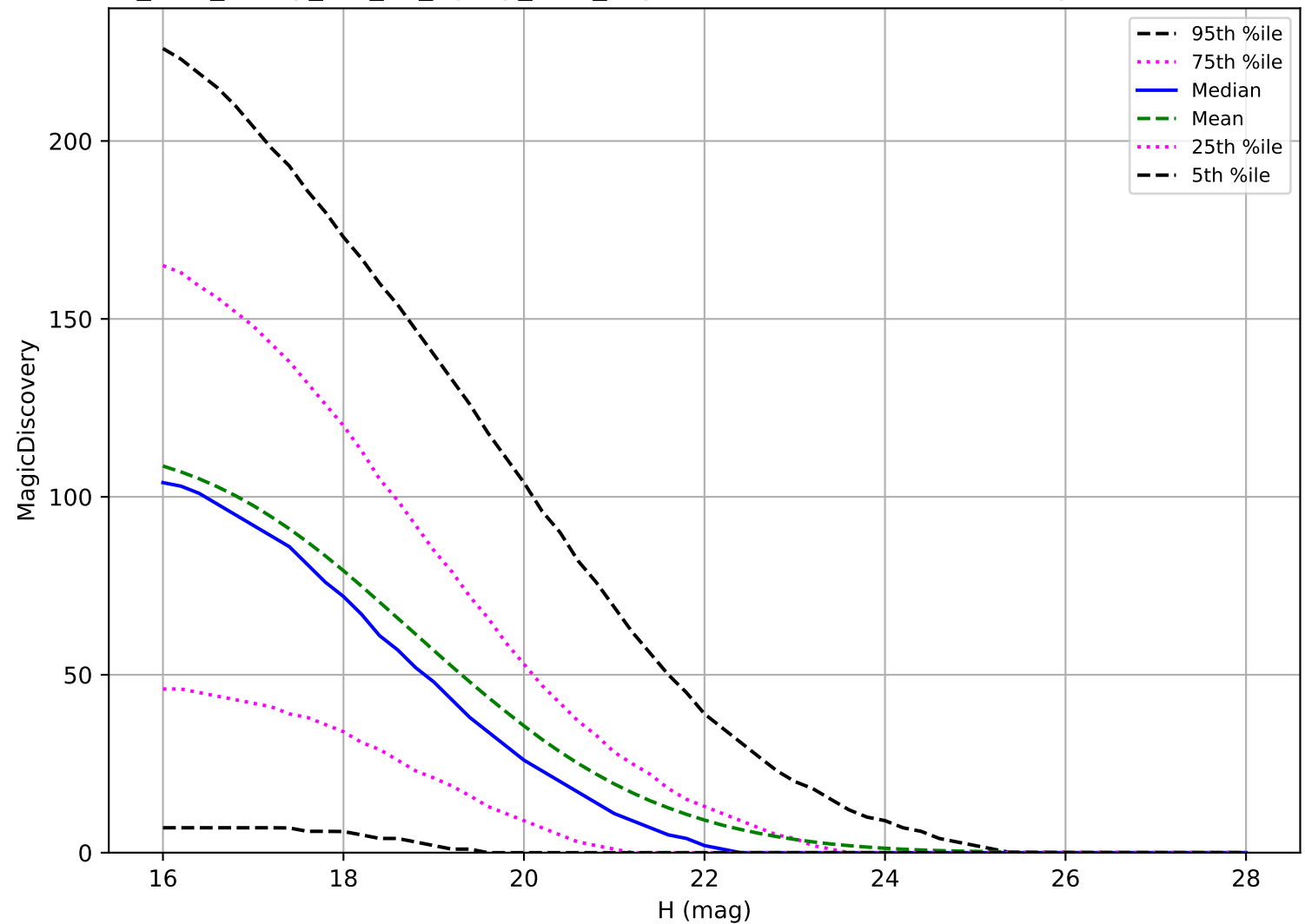
too_elab_heavy_r32_d3_ugrizy_v3.4_10yrs: PHA 6 detections in 60 nights detection loss
