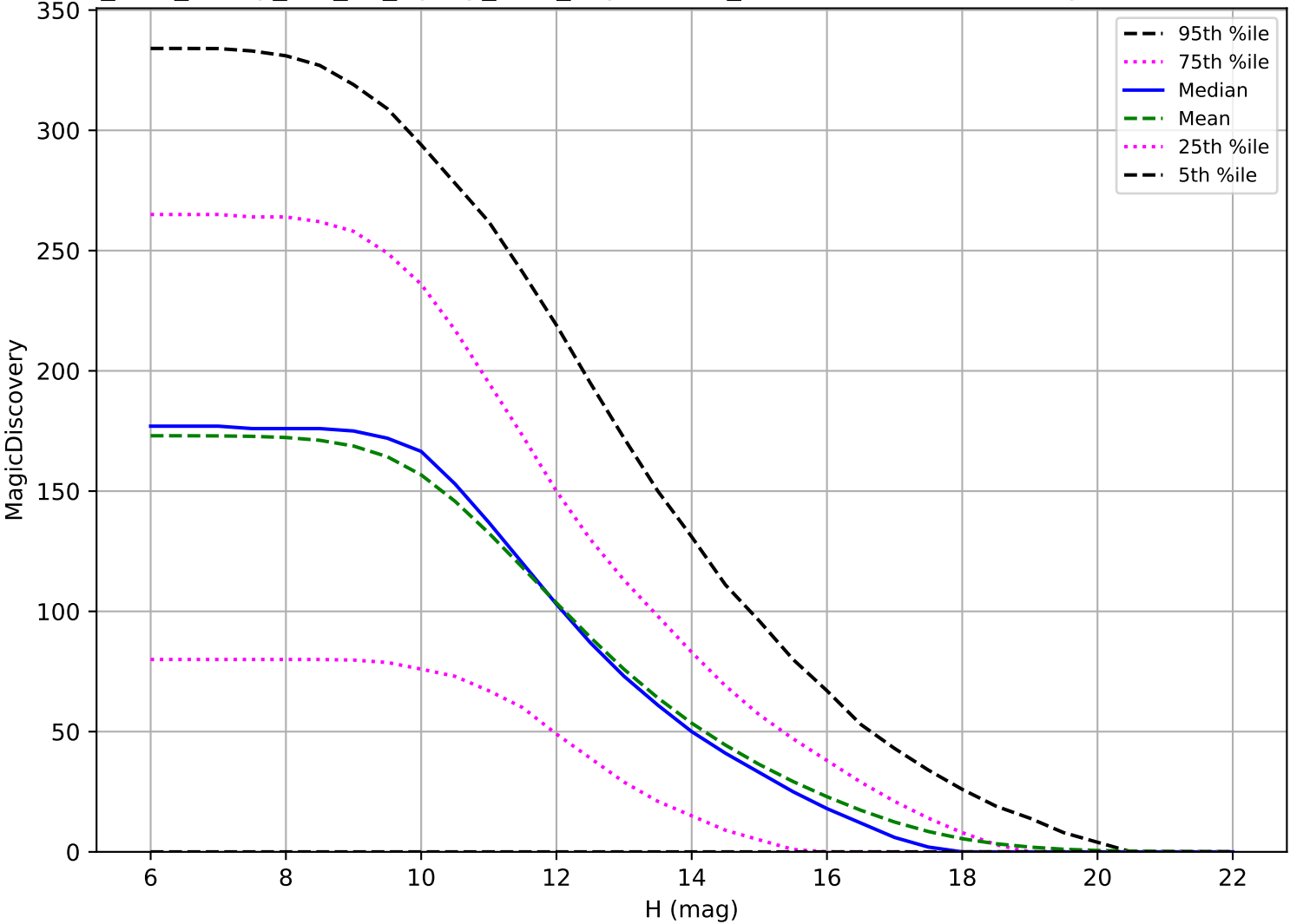
too_elab_heavy_r32_d3_ugrizy_v3.4_10yrs: OCC_r5 6 detections in 60 nights detection loss
