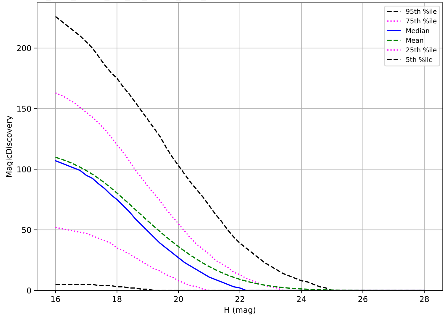
too_elab_heavy_r32_d3_ugrizy_v3.4_10yrs: NEO 6 detections in 60 nights detection loss
