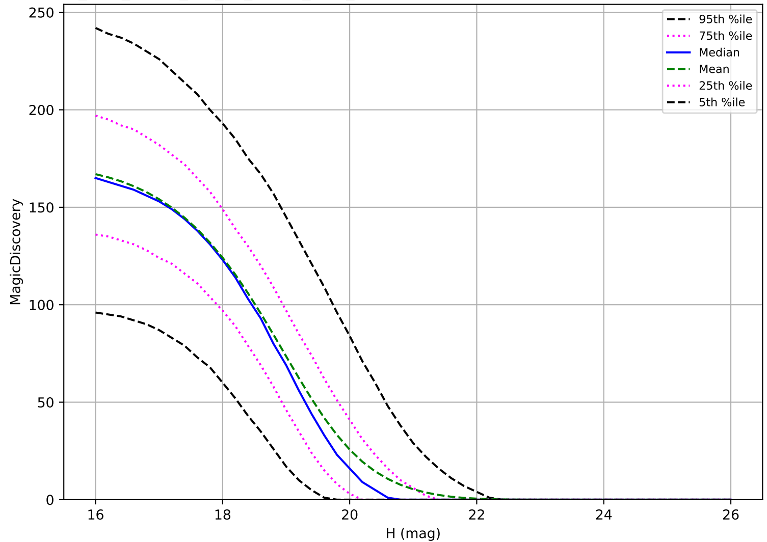
too_elab_heavy_r32_d3_ugrizy_v3.4_10yrs: MBA 6 detections in 60 nights detection loss
