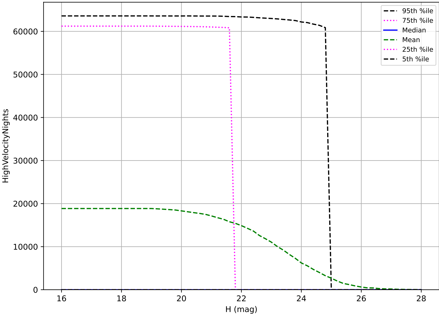
too_elab_heavy_r32_d3_ugrizy_v3.4_10yrs: NEO High velocity pair detection loss
