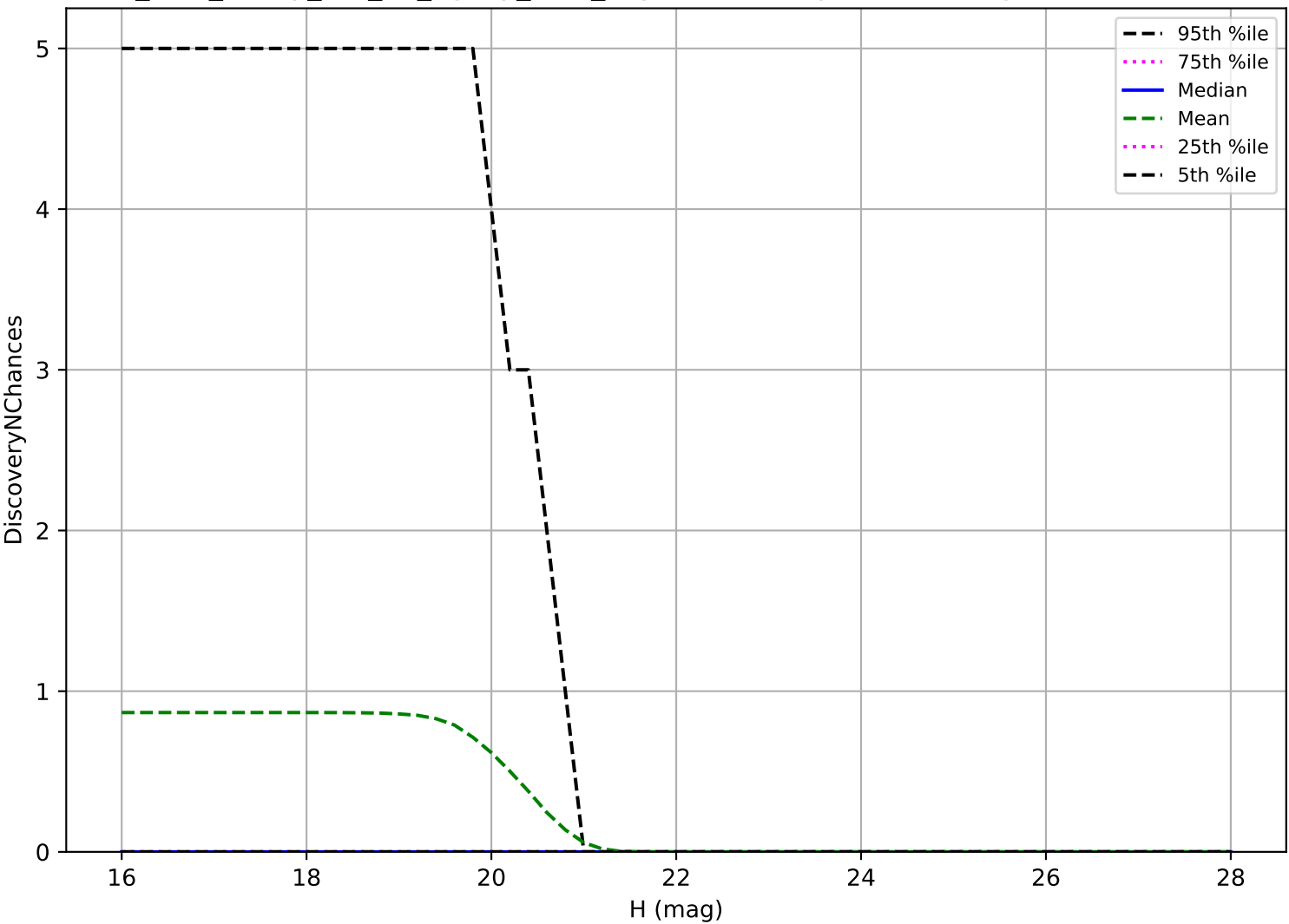
too_elab_heavy_r32_d3_ugrizy_v3.4_10yrs: Vatira 3 pairs in 15 nights detection loss
