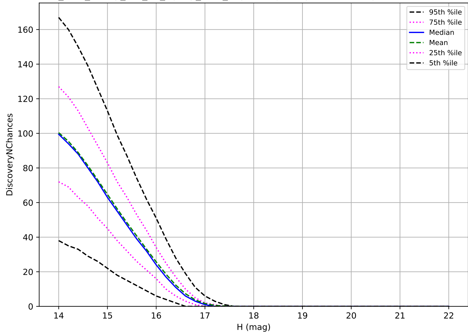
too_elab_heavy_r32_d3_ugrizy_v3.4_10yrs: Trojan 3 pairs in 15 nights detection loss
