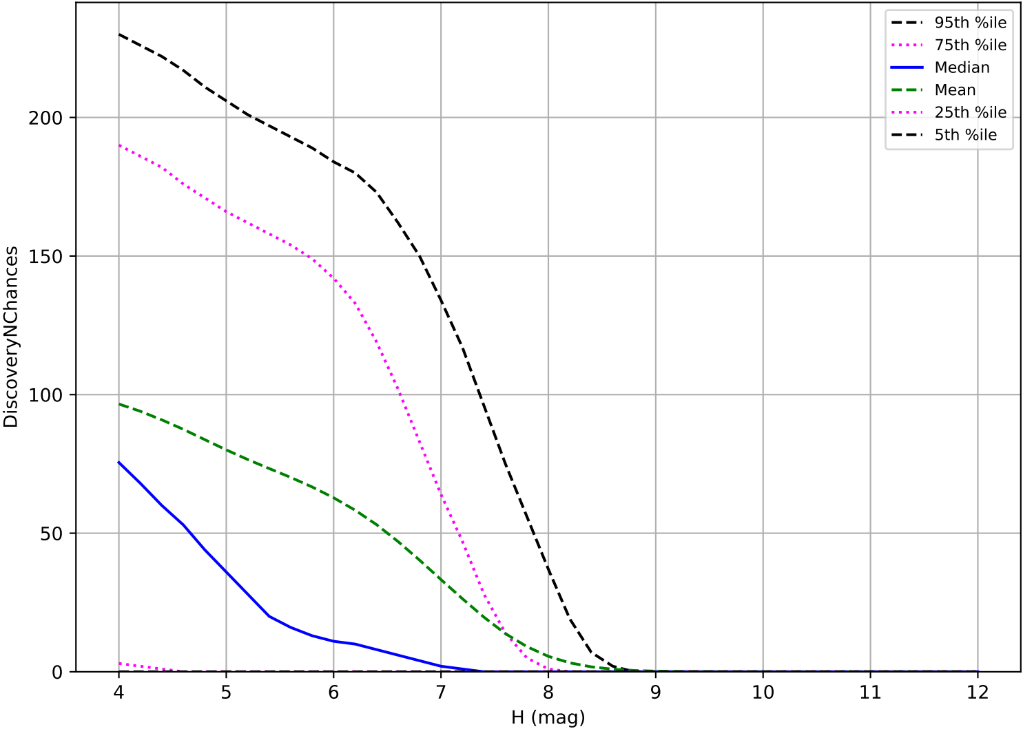
too_elab_heavy_r32_d3_ugrizy_v3.4_10yrs: TNO 3 pairs in 15 nights detection loss
