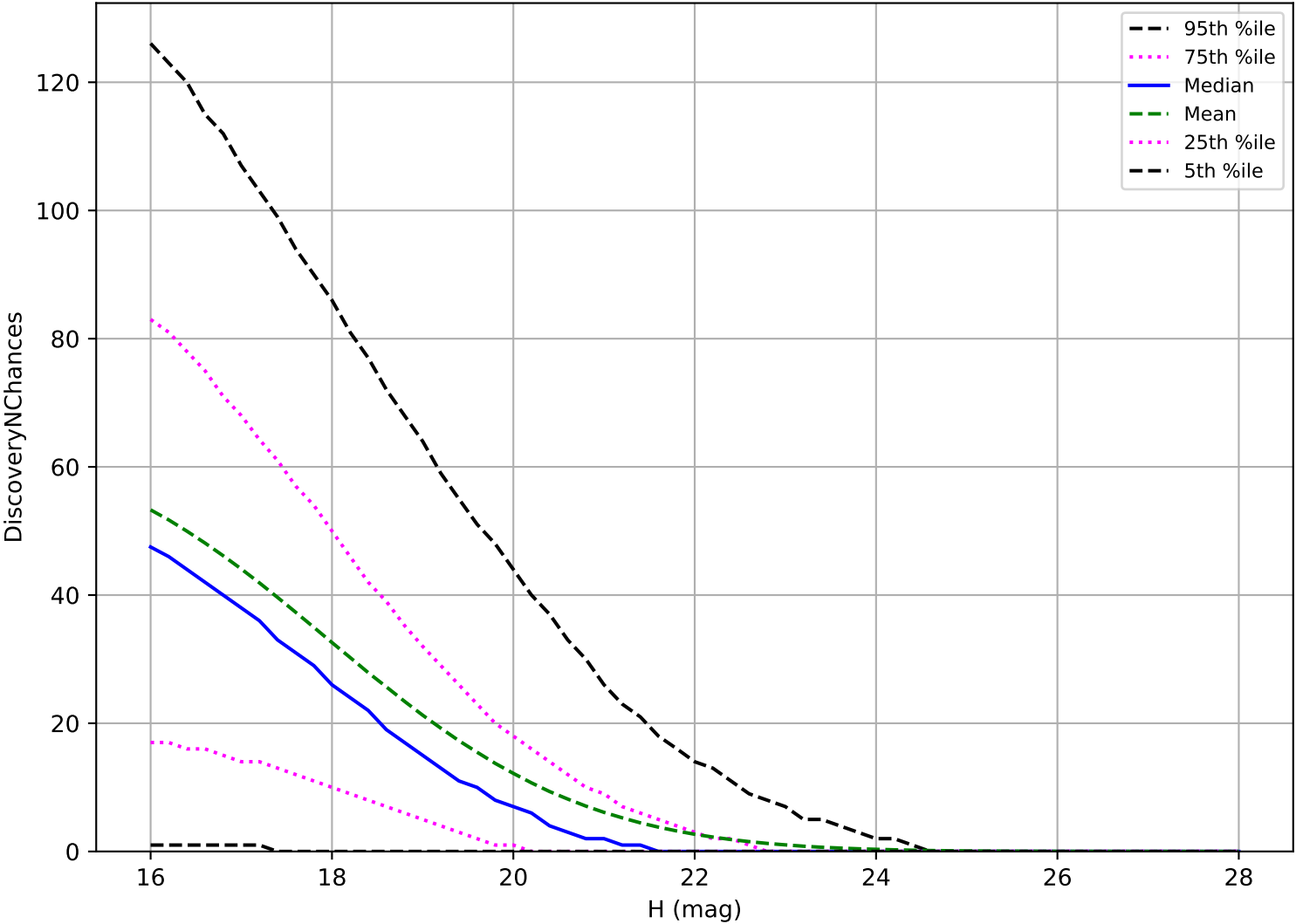
too_elab_heavy_r32_d3_ugrizy_v3.4_10yrs: PHA 3 pairs in 15 nights detection loss
