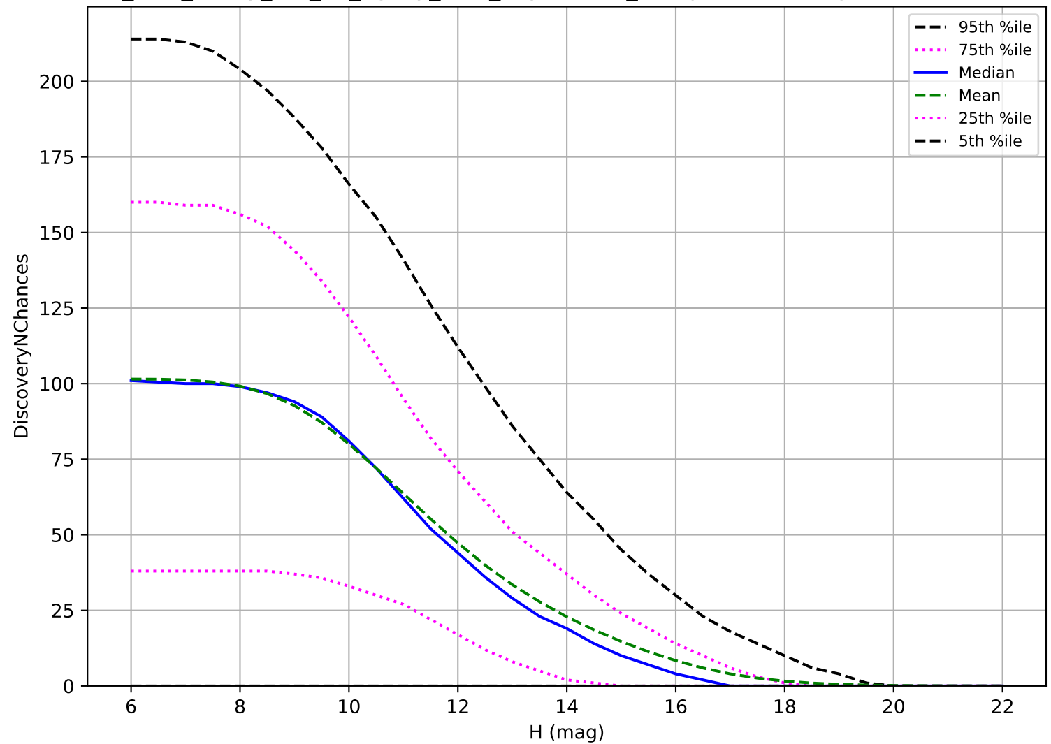
too_elab_heavy_r32_d3_ugrizy_v3.4_10yrs: OCC_r5 3 pairs in 15 nights detection loss
